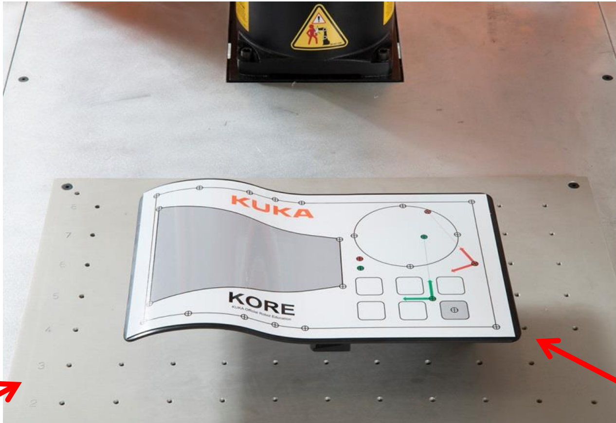
Referenced Mounting Sub-Plate
